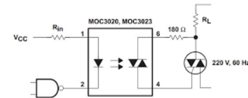
Figure 5. Resistive Load
